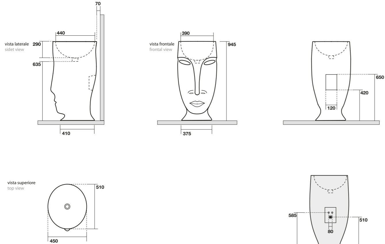
4740 Lavabo freestanding Moloco scarico a parete Freestanding washbasin Moloco wall outlet
