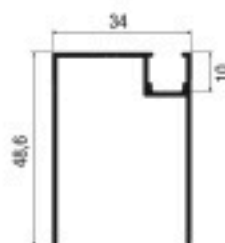
Marco lateral
