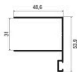
Marco lateral
